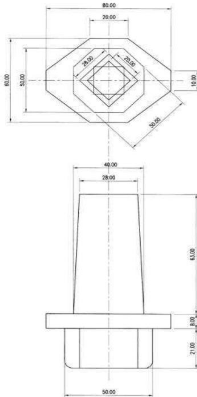
ANNEXE C Dimensions of operating cap Type B
